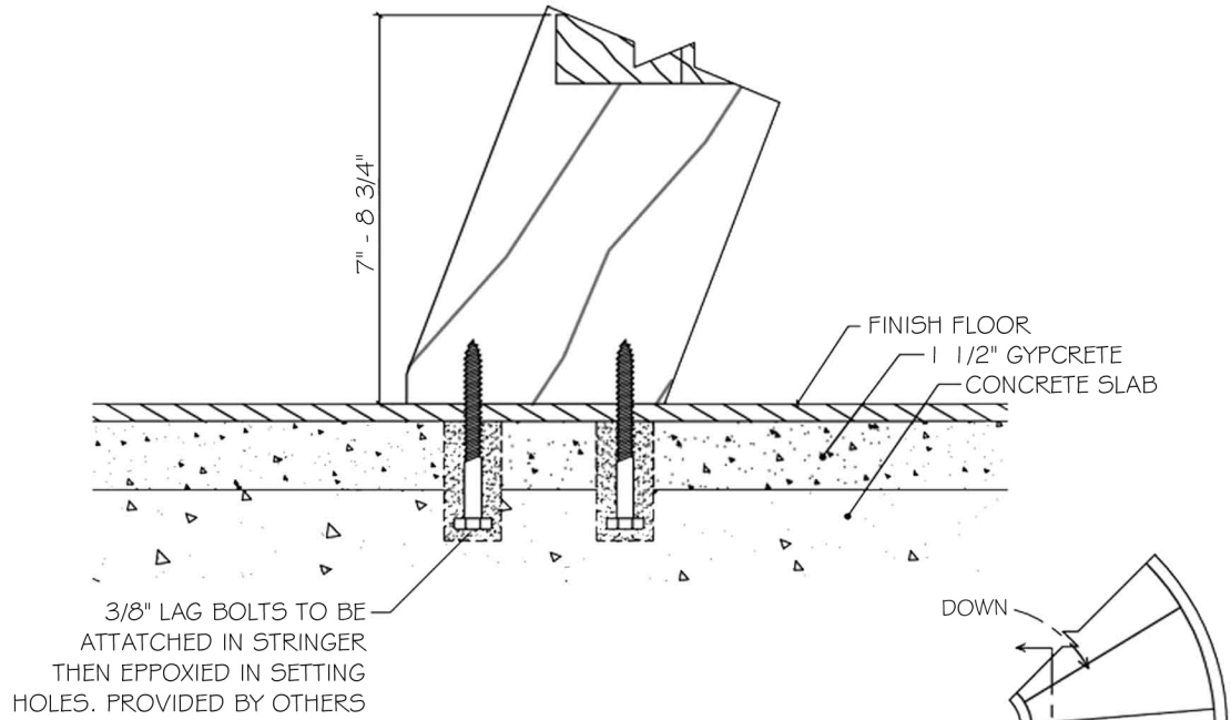
TYPICAL INNER STRINGER SECTION @ FLOOR ANCHOR BOLT DETAIL
